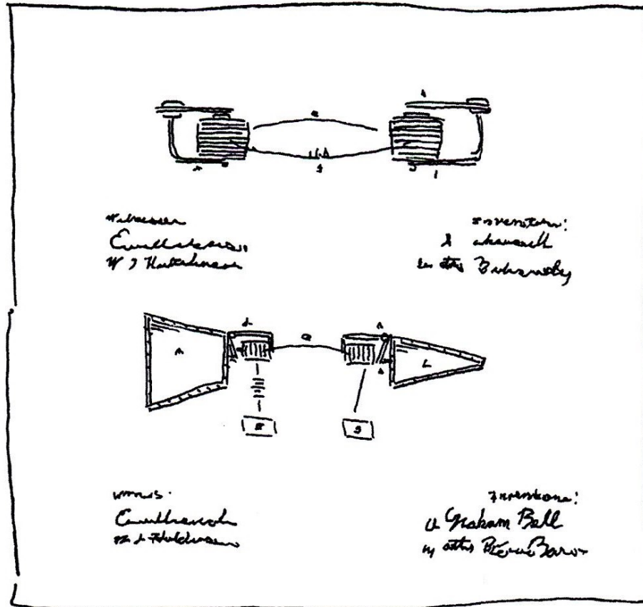
BELL'S TELEPHONE DIAGRAM
